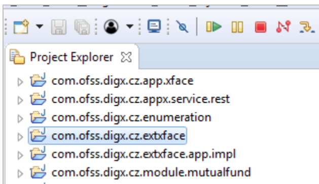
Figure 2 Project structure
